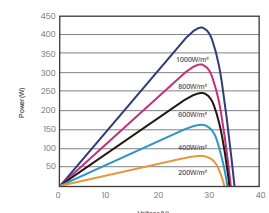
P-V CURVES OF PV MODULE(425W)
