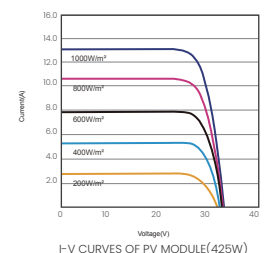
I-V CURVES OF PV MODULE(425W)
