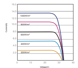
I-V CURVES OF PV MODULE(435W)
