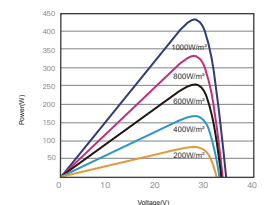
P-V CURVES OF PV MODULE(435W)
