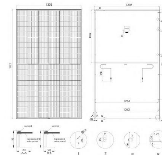
Fig. 1: External dimensions (inmm) and components for SR-60MAXH
