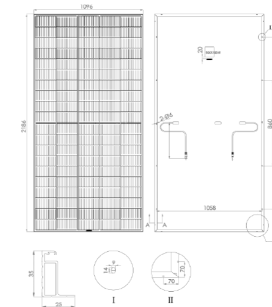
External dimensions (inmm) and components for SR-50MAXH
