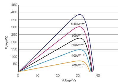
P-V CURVES OF PV MODULE(385W)
