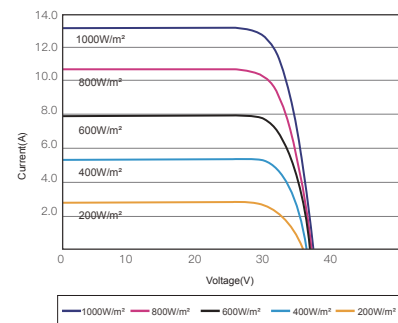
I-V CURVES OF PV MODULE(385W)
