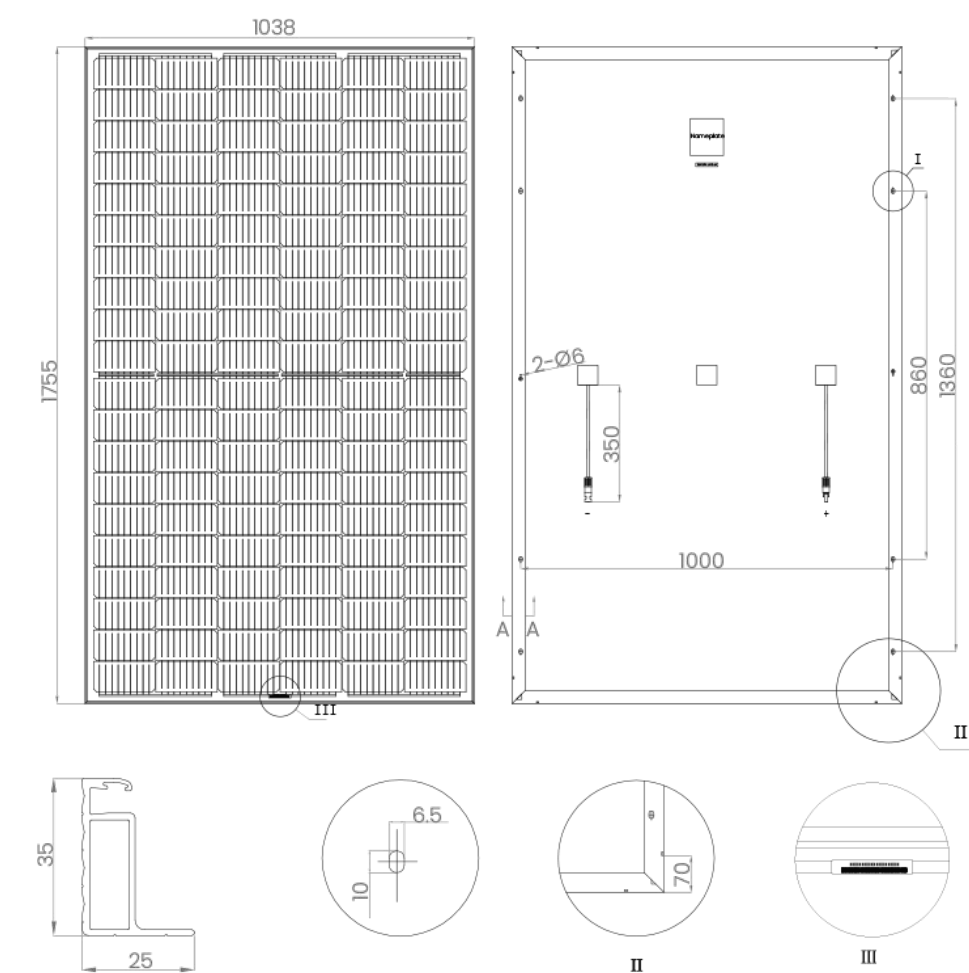
Fig. 2: External dimensions (in mm) and components for SR-M660-HLP
