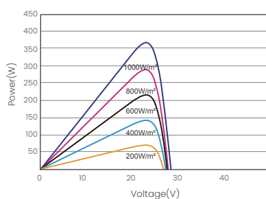
P-V CURVES OF PV MODULE(360W)
