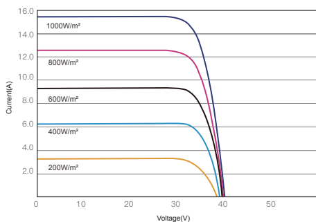
I-V CURVES OF PV MODULE(610W)
