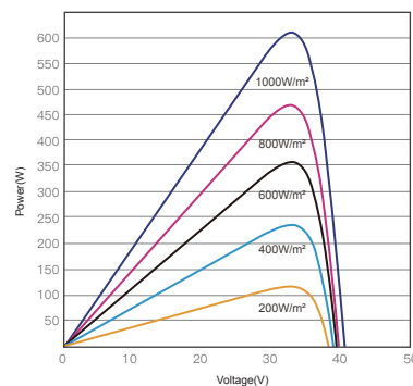
P-V CURVES OF PV MODULE(610W)
