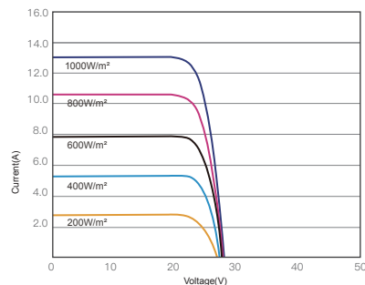
I-V CURVES OF PV MODULE(375W)
