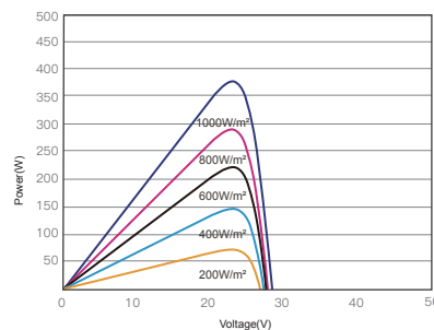
P-V CURVES OF PV MODULE(375W)
