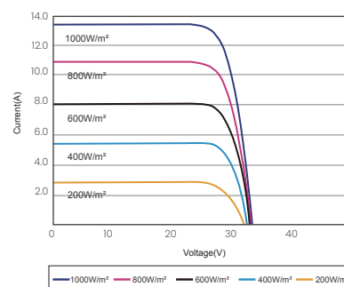
I-V CURVES OF PV MODULE(440W)
