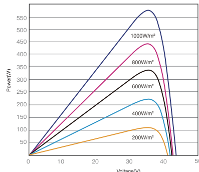
P-V CURVES OF PV MODULE(575W)
