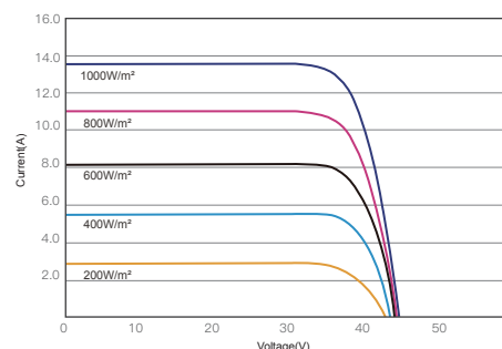
I-V CURVES OF PV MODULE(590W)
