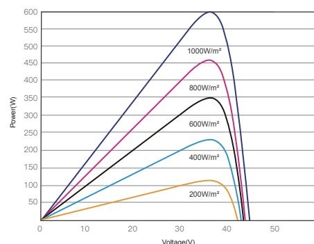
P-V CURVES OF PV MODULE(590W)
