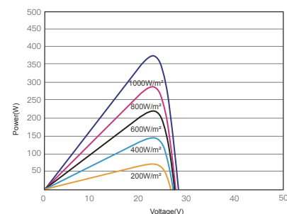
P-V CURVES OF PV MODULE(370W)
