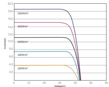
I-V CURVES OF PV MODULE(595W)
