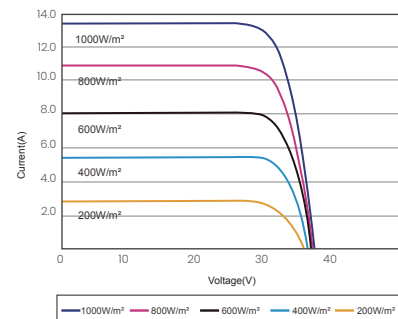
I-V CURVES OF PV MODULE(405W)
