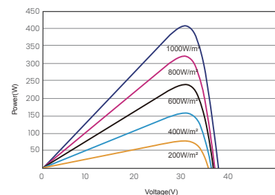
P-V CURVES OF PV MODULE(405W)
