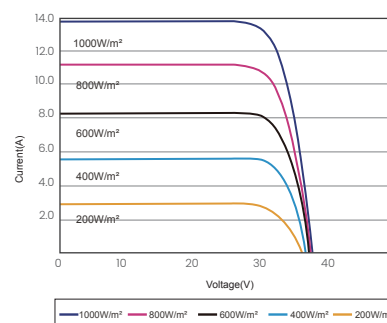
I-V CURVES OF PV MODULE(410W)
