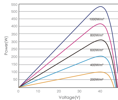
P-V CURVES OF PV MODULE(540W)
