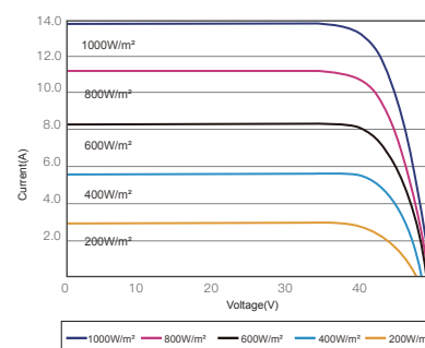
I-V CURVES OF PV MODULE(540W)
